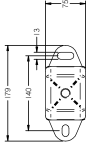
AVM MOUNT DETAILS
