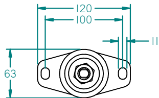
MOUNT DETAILS
